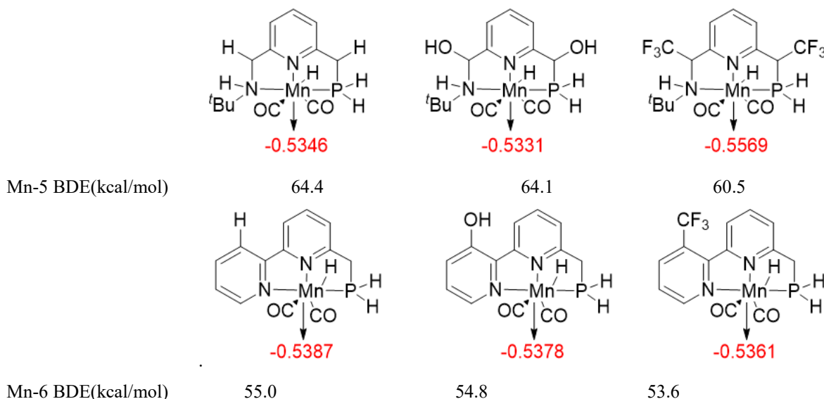
Fig. 8: The natural charge data on Mn atoms in Mn-5 and Mn-6 molecules.
