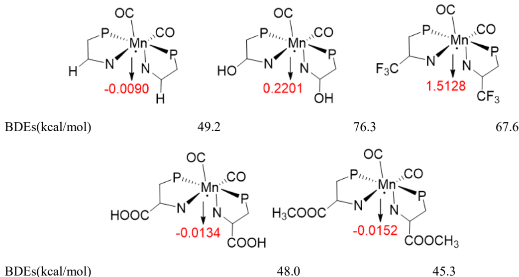
Fig. 6: The Spin density data on Mn in free radicals of R=-H, -OH, -CF 3 , -COOH and -COOCH 3 .
